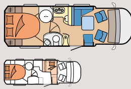
T65 GQ
