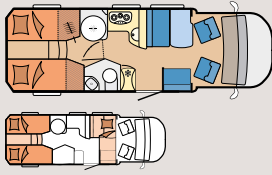
T70 GE
