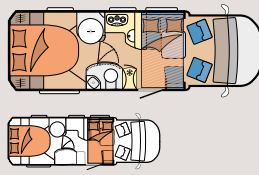
T65 HGQ
