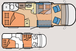
T65 HFL
