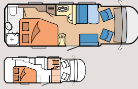
T70 F
