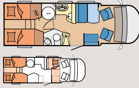
T70 GE
